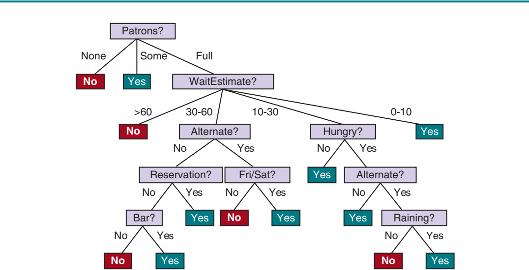
Figure 19.3 A decision tree for deciding whether to wait for a table.
